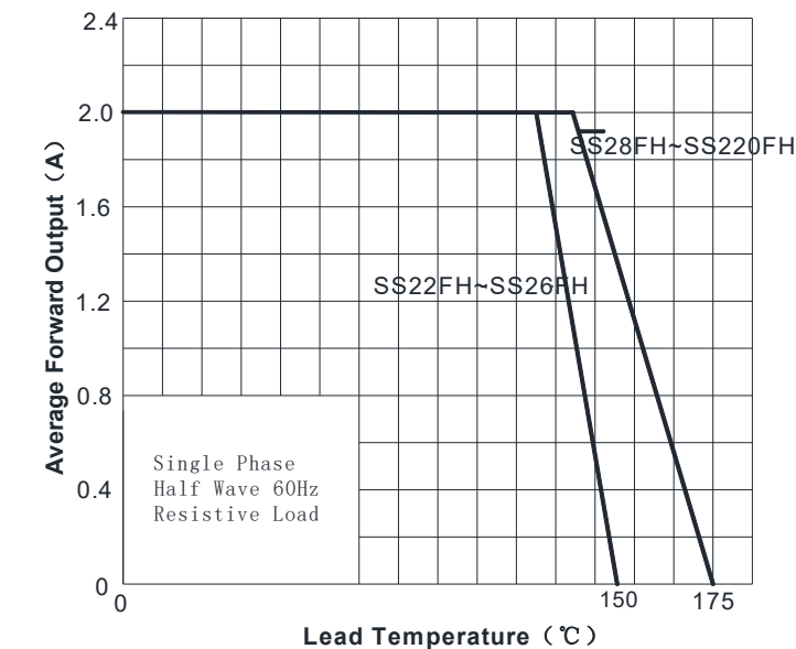
FIG1:Io-TL Curve
